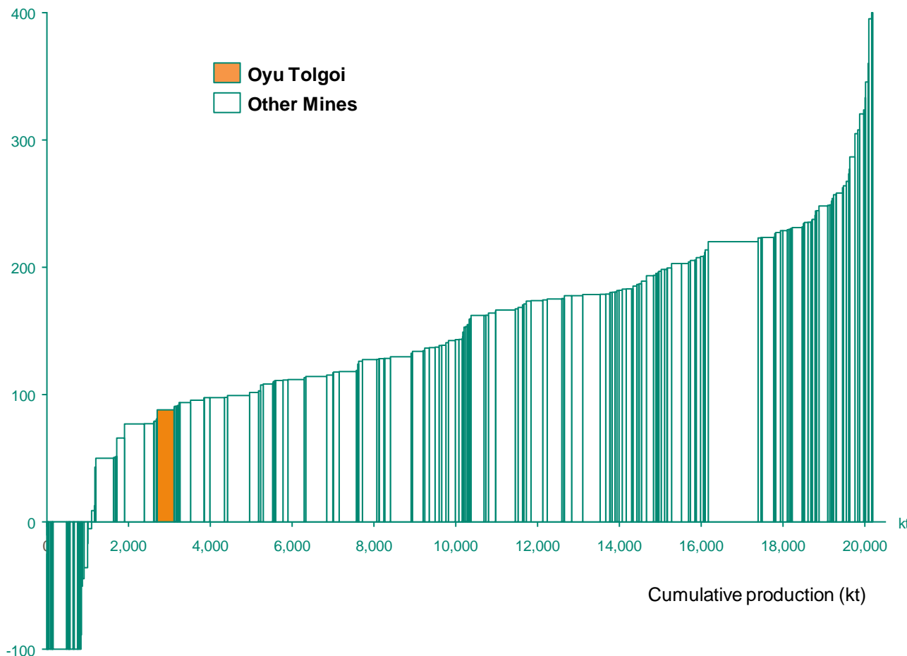
Copper mine C1 cost curve in 2020 (c/lb, 2014$)
